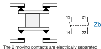
The 2 moving contacts are electrically separated
