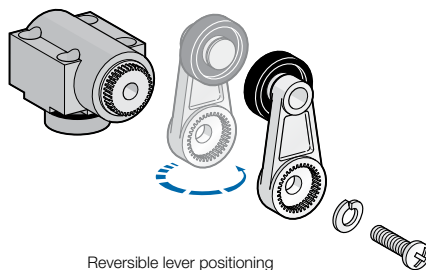
Reversible lever positioning
